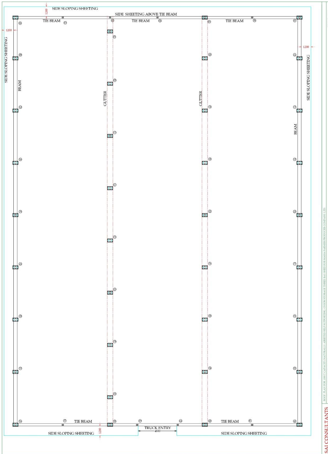
Drawing: Gutter and Side Sheeting
